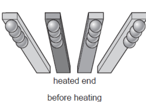
▲ Comparing four good thermal conductors. Ten minutes or so after the boiling water has been tipped into the tank, the length of melted wax shows which material is the best conductor.
